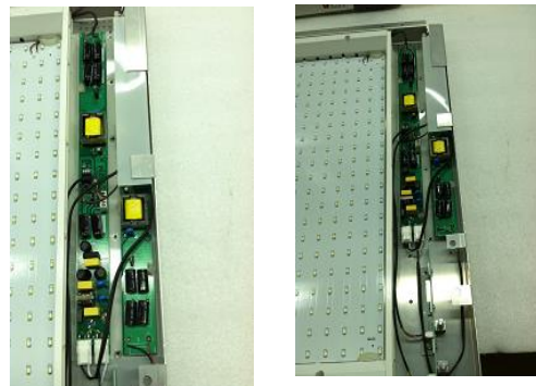
Switching Mode Power Supplier (SMPS) Inverter Separate Dimming Control Board by On/Off Switch
